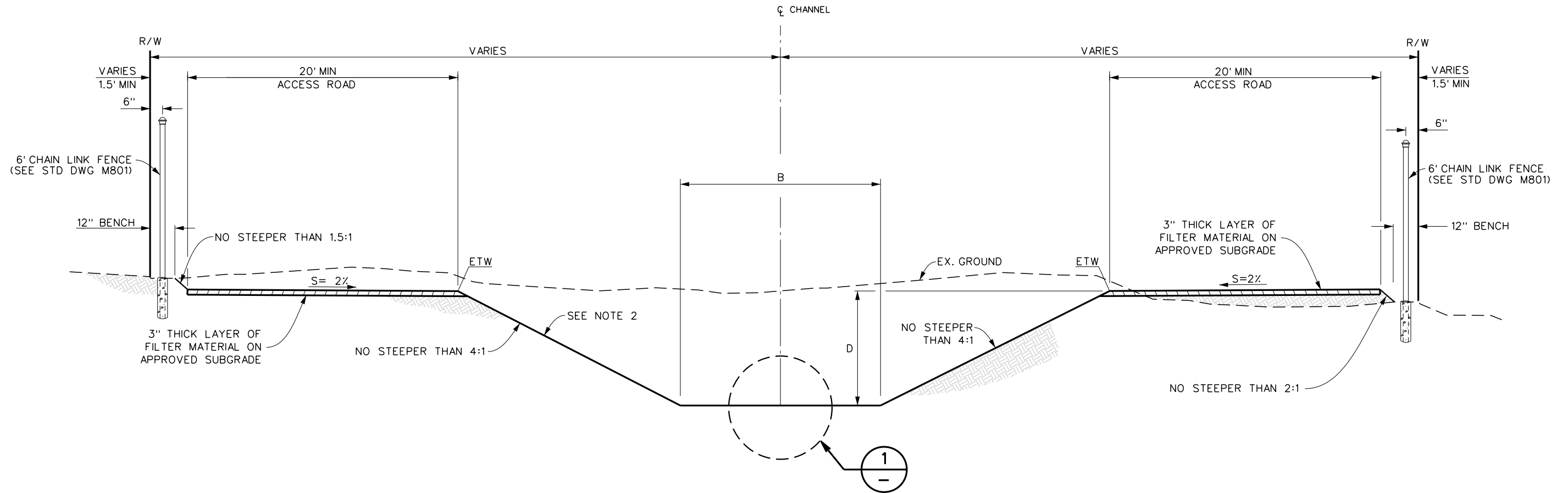
TYPICAL CHANNEL SECTION NTS
