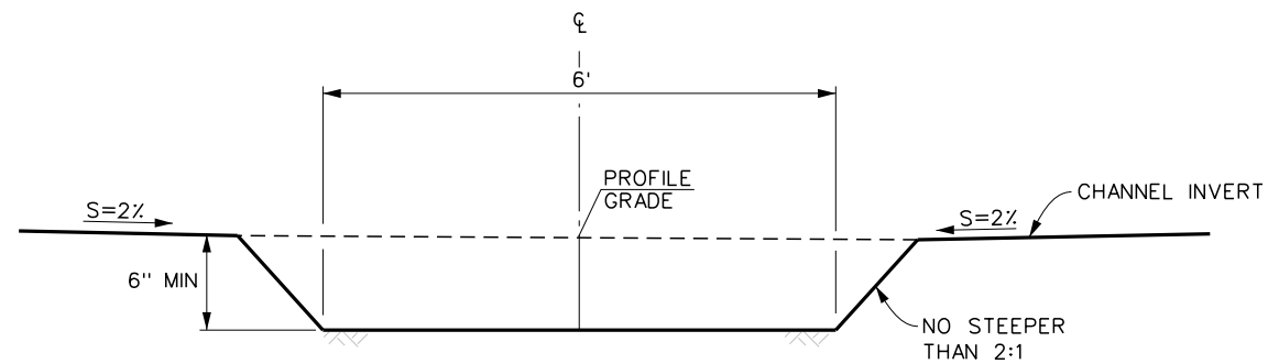
LOW FLOW DETAIL 1 FOR B \geq 50' NTS
