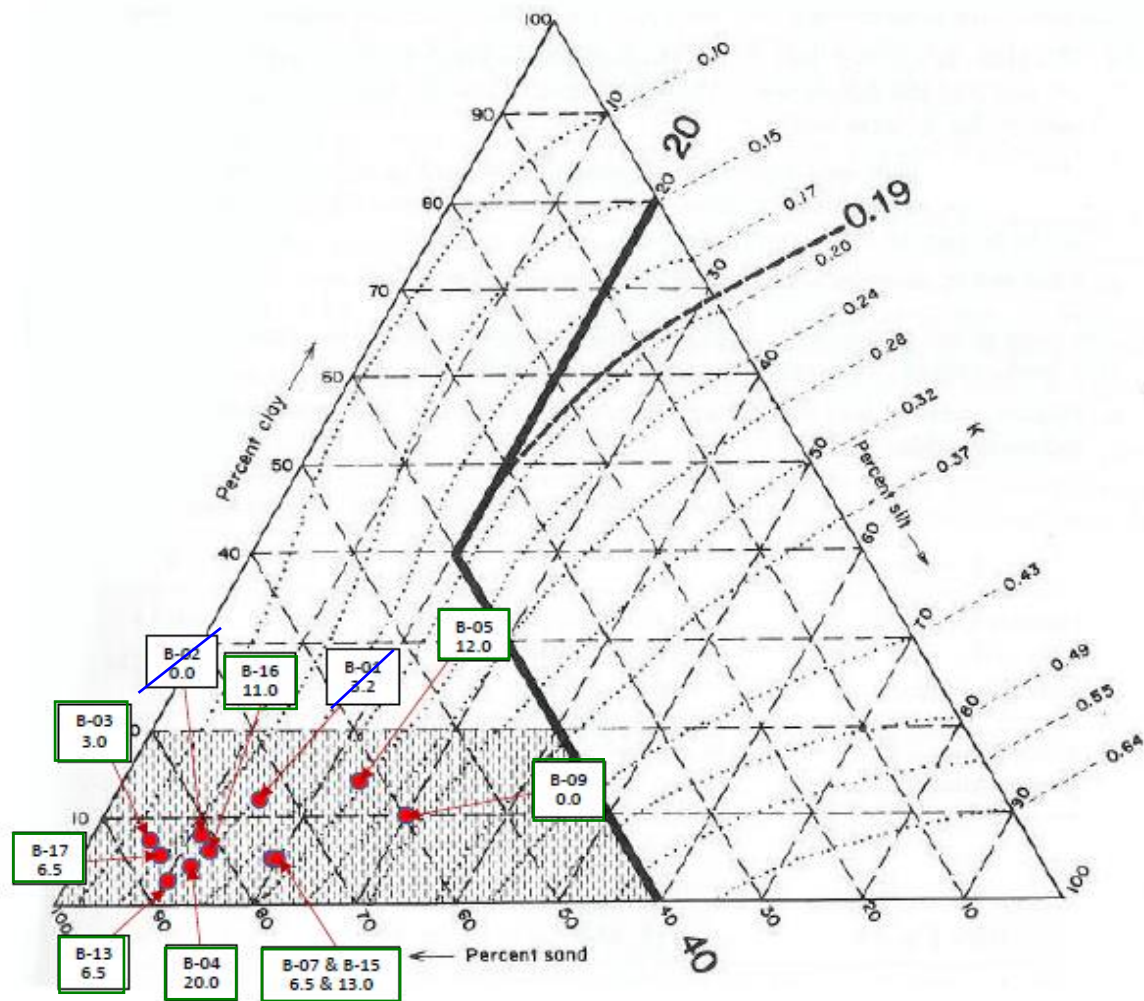
Erickson triangular nomograph used to estimate soil erodibility (K) factor. USDA nomograph from Erickson 1977 as referenced by Goldman et al., 1986.
